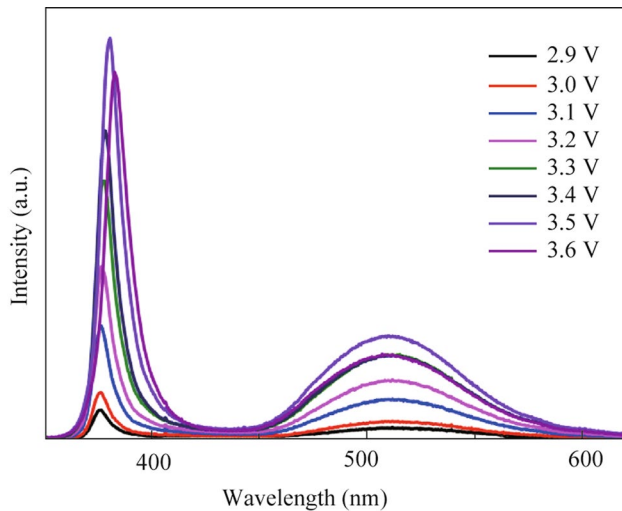
Fig. 8 Voltage-dependent photoluminescence study of an optimized remote phosphor (BSSP film-50 mg)
