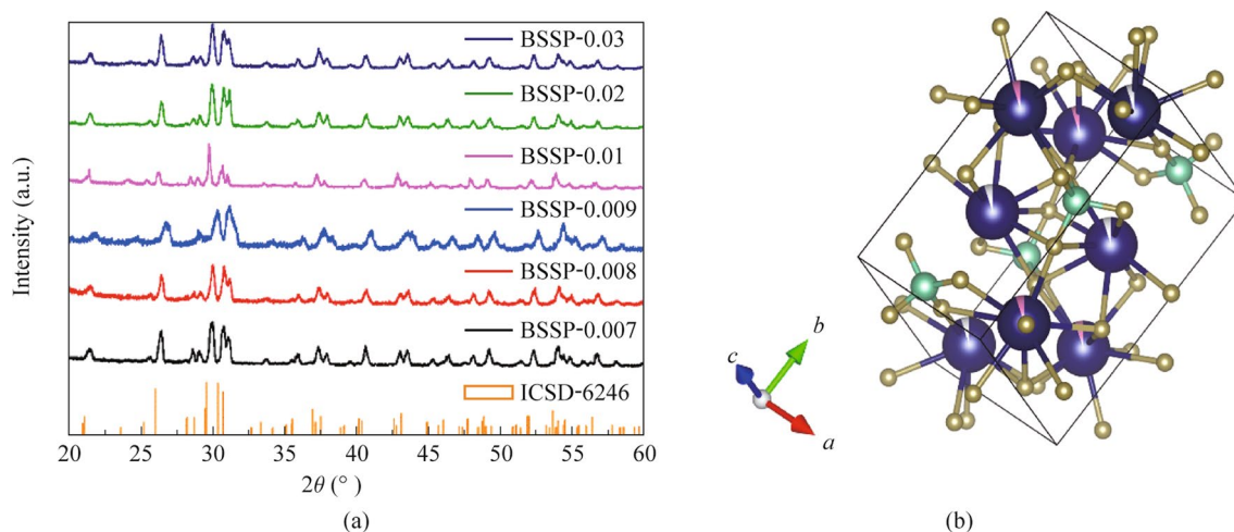
Fig. 1 a X-ray diffraction patterns of BSSP-0.007, 0.008, 0.009, 0.01, 0.02, and 0.03 phosphors. b Schematic crystal structure of BSSP phosphor
