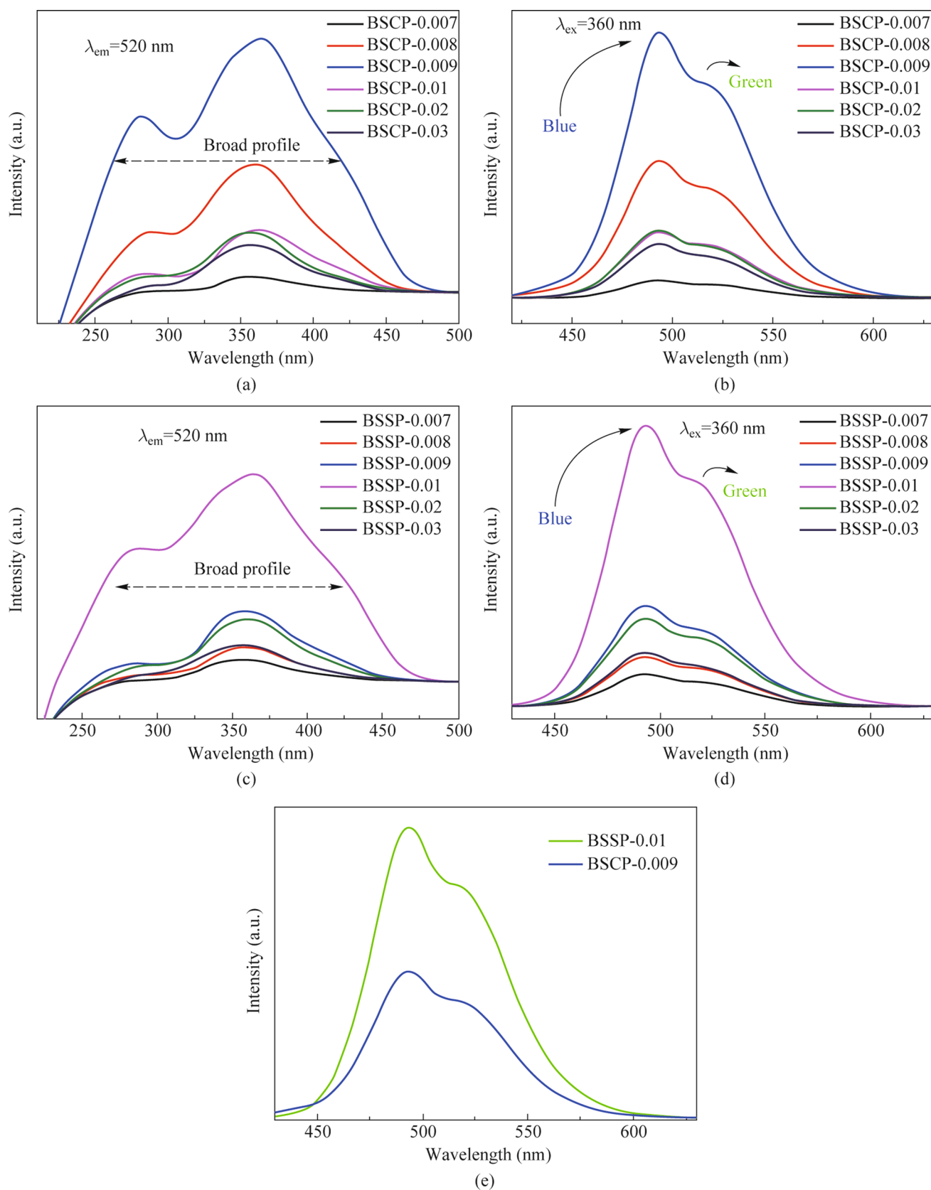
Fig. 2 a and c Photoluminescence excitation spectra of BSSP & BSCP (–0.007, 0.008, 0.009, 0.01, 0.02, and 0.03). b and d Photoluminescence emission spectra of BSSP & BSCP (–0.007, 0.00, 0.009, 0.01, 0.02, and 0.03). e Comparative study of photoluminescence emission spectra of BSSP-0.01 and BSCP-0.009
