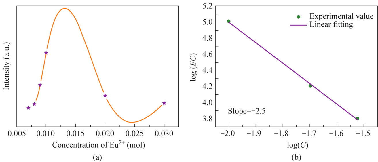
Fig. 3 a Plot of the concentration of \text{Eu}^{2+} vs intensity. b Energy transfer mechanism plot of \log(C) vs \log(I/C)
