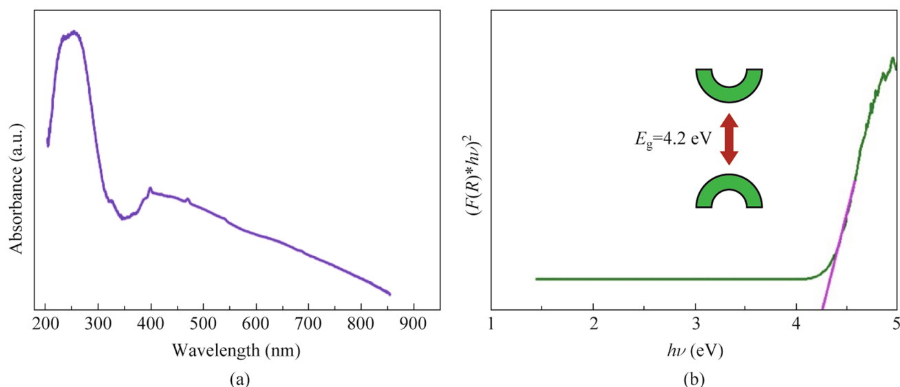
Fig. 5 a UV-vis spectra. b Band gap plot of BSSP-0.01 phosphor
