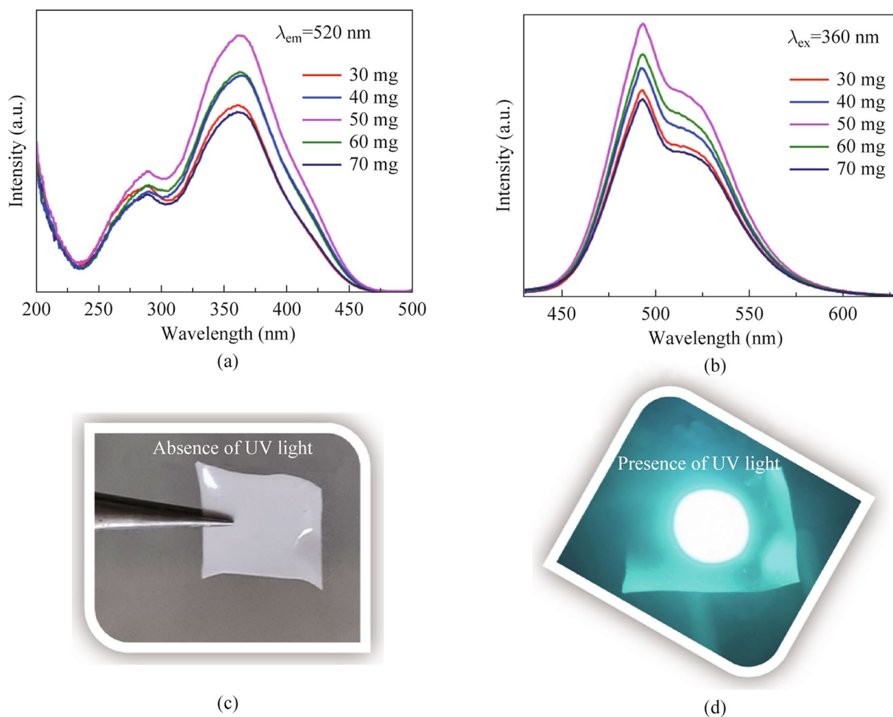
Fig. 7 a and b Study between the weight of the phosphor and the change in luminescence intensity. c and d Illumination effect of the prepared BSSP film in the presence and absence of UV light
