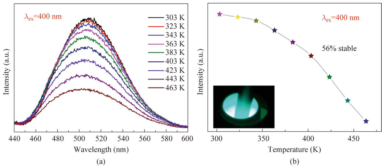
Fig. 4 a Temperature-dependent photoluminescence spectra of BSSP-0.01 phosphor in the temperature range of 303–463 K. b Relationship between temperature and PL intensity, inset: Emission color of the phosphor under 400 nm excitation
