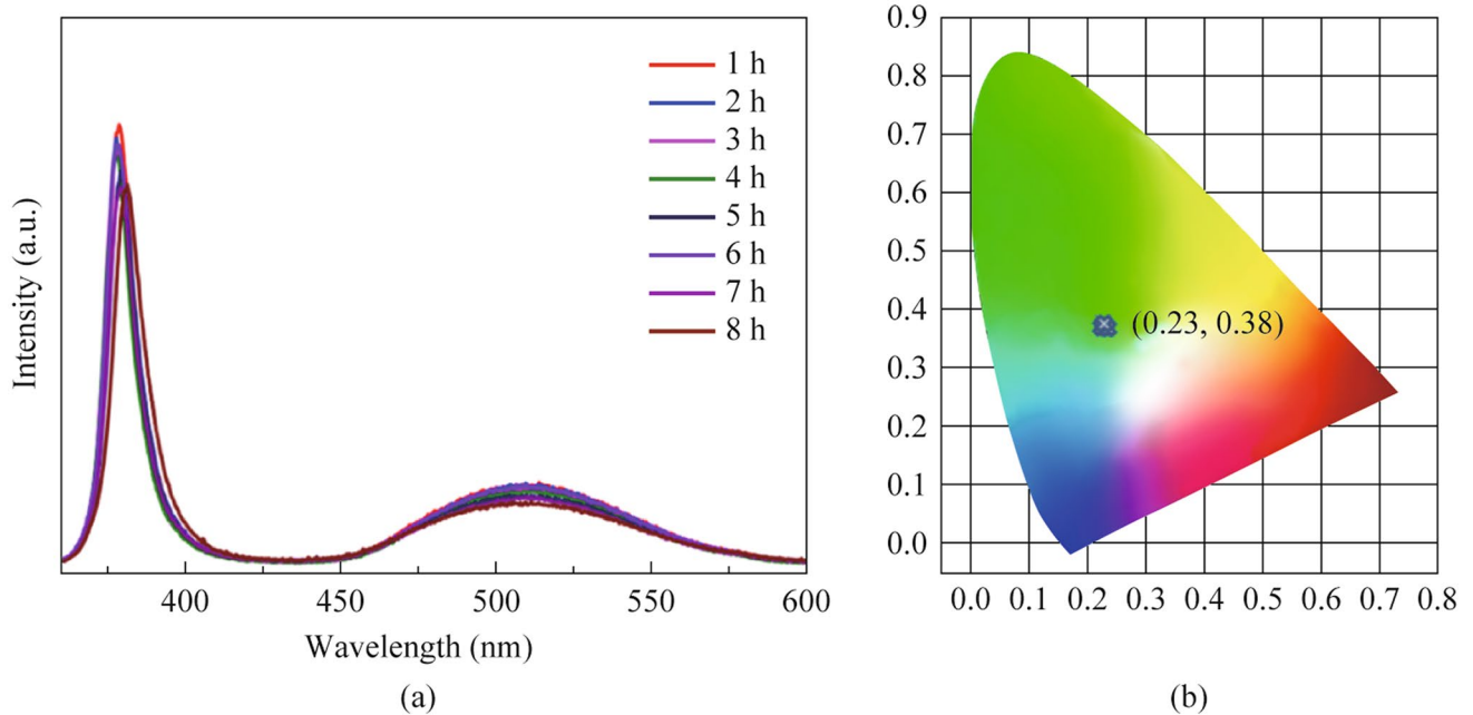
Fig. 9 a Photoluminescence spectra. b CIE diagram of the optimized BSSP film-50 mg driven by 380 nm LED over a time
